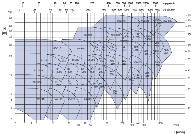
SELECTION CHART at 1.450 r.p.m.
